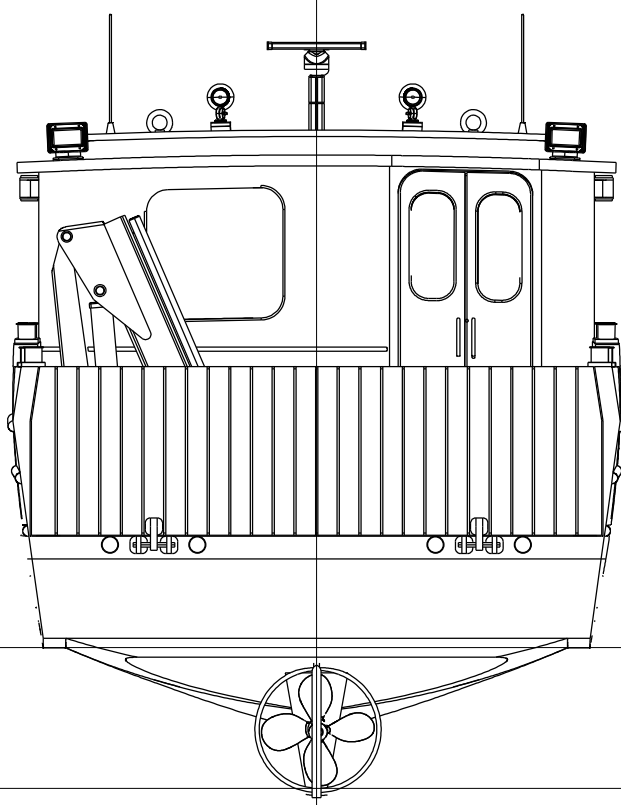
Stern view (Widok od rufy)
